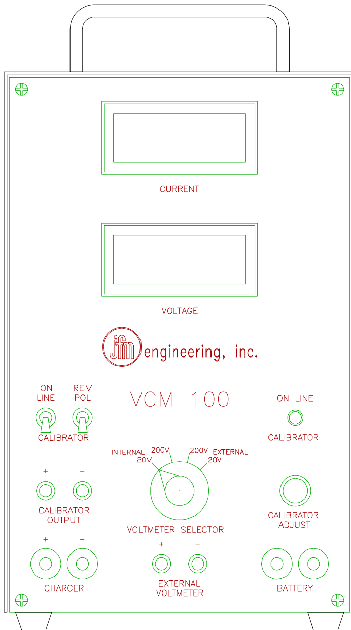
Figure 1 – Front View
